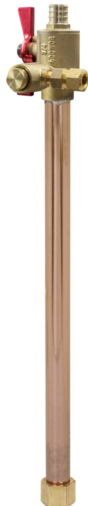
Sioux Chief Thermal Expansion Relief Valves For in-line F1807 PEX connection (top); or as part of a preformed copper water heater connector (above)
